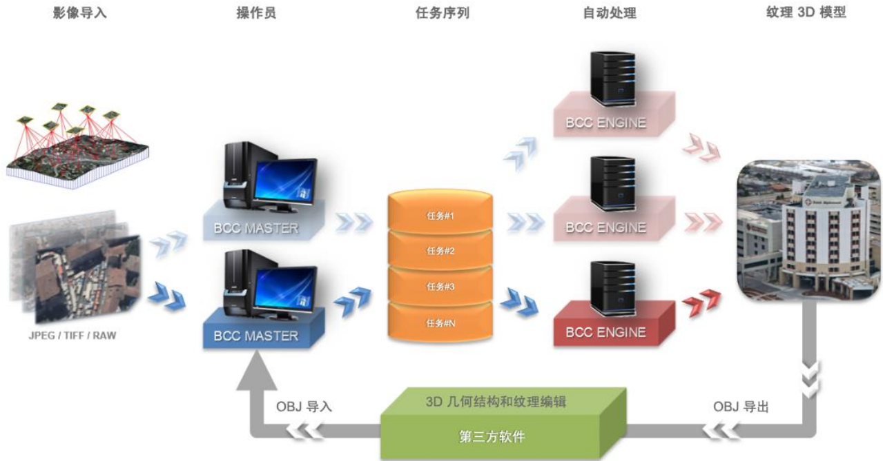
图9: ContextCapture workflow
